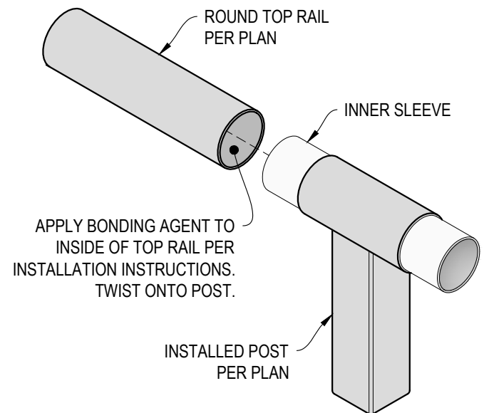
B TOP RAIL INSTALLATION - ROUND DETAIL
