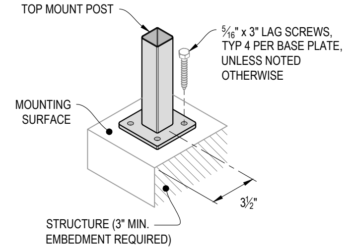
C TYPICAL POST MOUNTING - TOP MOUNT DETAIL
