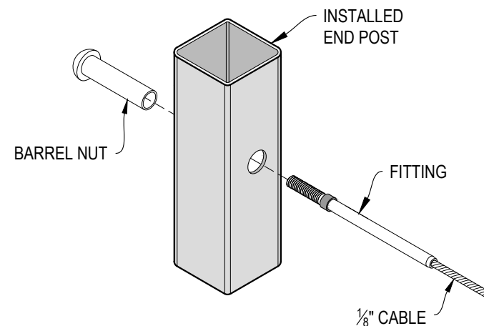
F FITTING INSTALLATION - BARREL NUT DETAIL
