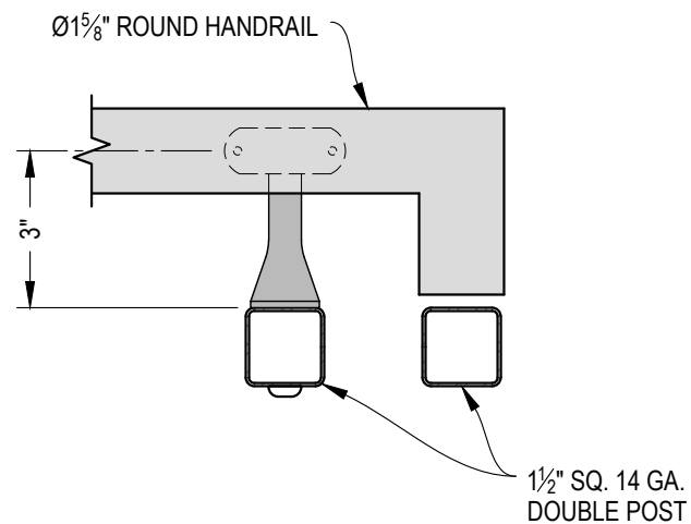
B TYPICAL HANDRAIL RETURN - ROUND DETAIL
