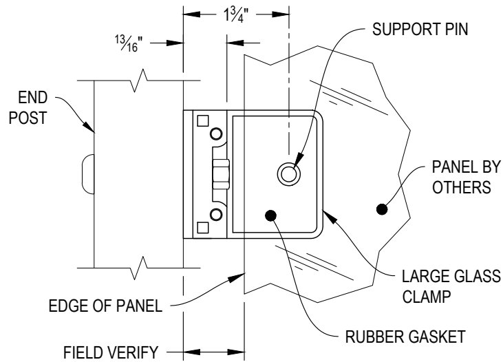
A TYPICAL HANDRAIL RETURN - FLAT DETAIL
