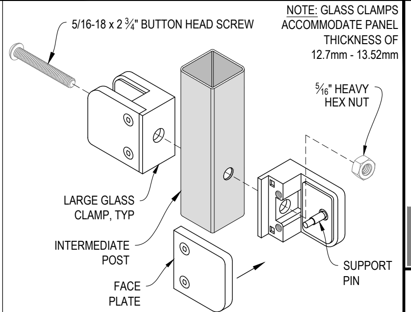
C INTERMEDIATE POST GLASS CLAMP INSTALLATION - LARGE DETAIL
